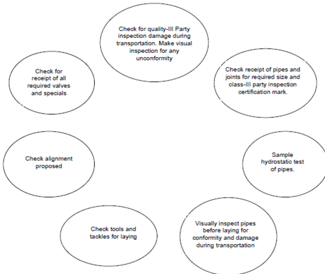
Figure 8.1 (b) CHECKS FOR PREPARATION WORKS BEFORE LAYING WATER SUPPLY PIPE LINES
