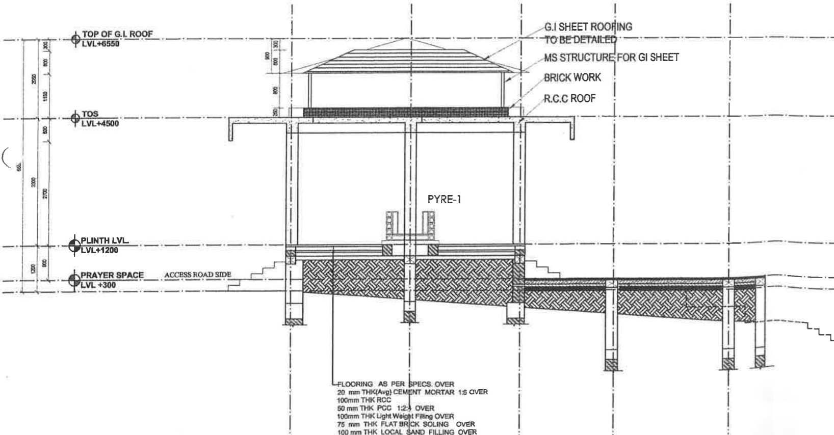
SECTION BB'
