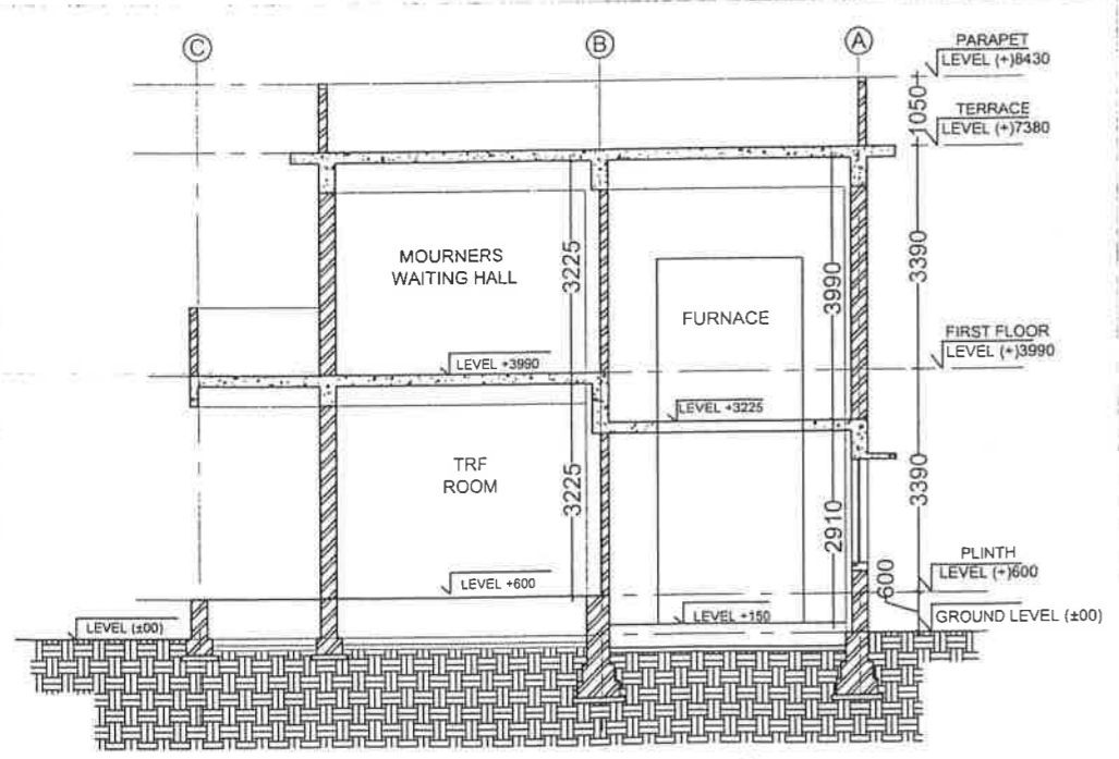
SECTION-XX
